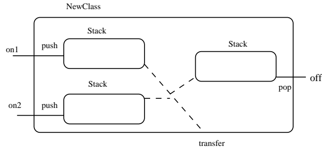
Figure 7: A Dependency Example
