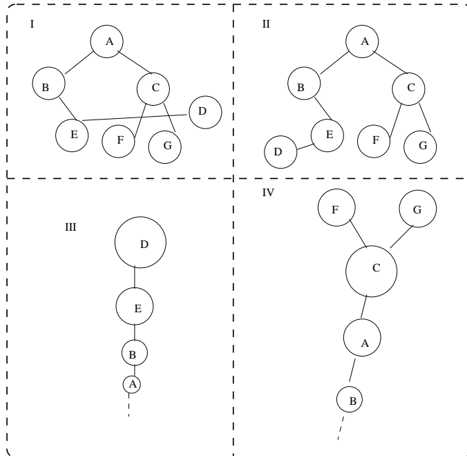
Figure 9: Pretty Pictures
