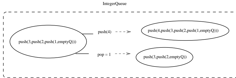
Figure 13: A User Defined Visualisation
