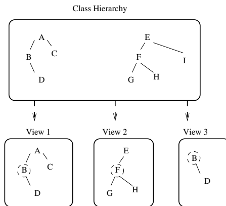
Figure 10: Visual Abstraction In A Class Hierarchy
