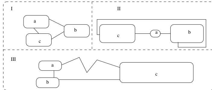
Figure 8: Whitespace Examples
